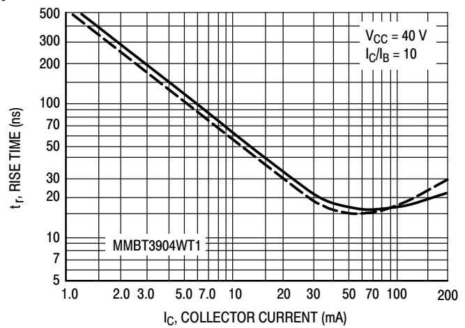
Figure 4. Rise Time
