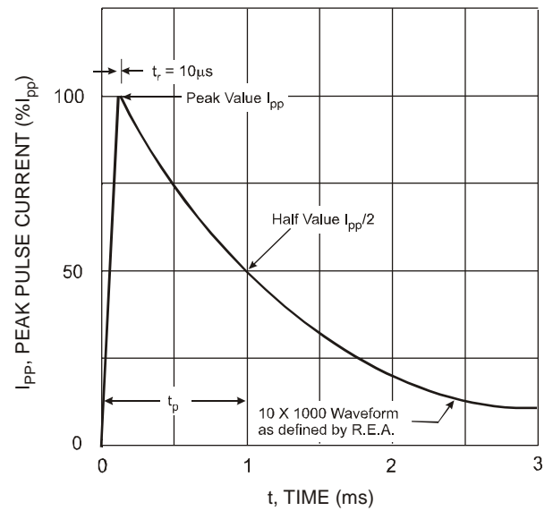
Figure 4. Pulse Waveform
