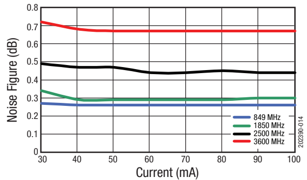
Figure 14. Evaluation Board NF vs Quiescent Current Over Frequency Using Band-Specific BOM
