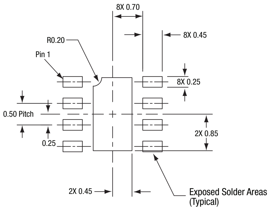
Figure 25. SKY67151-396LF PCB Layout Footprint (Top View)
