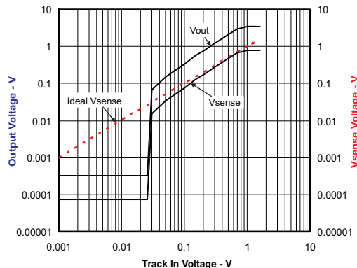
Figure 50. Tracking Performance
