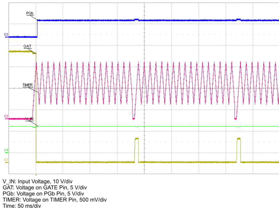
Figure 28. Auto-Restart Cycle Timing
