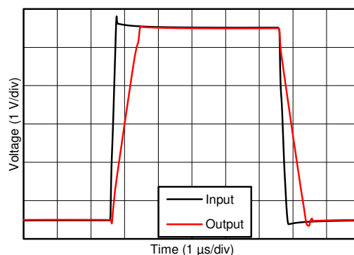
Figure 5-26. Overload Recovery
