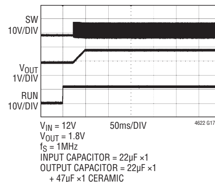
Start-Up into Pre-Biased Output
