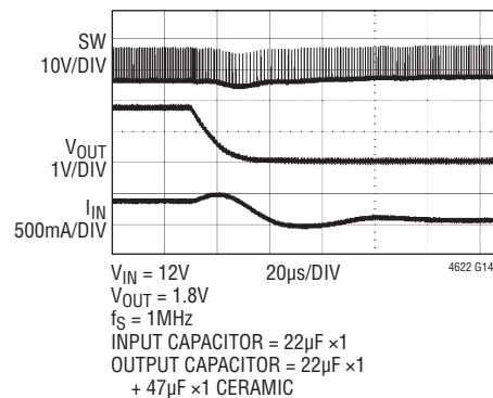
Short-Circuit with 2.5A Load Current Applied
