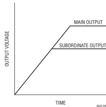
Figure 6. Output Coincident Tracking Waveform
