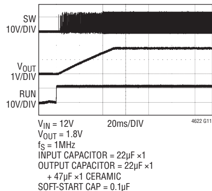
Start-Up with No Load Current Applied
