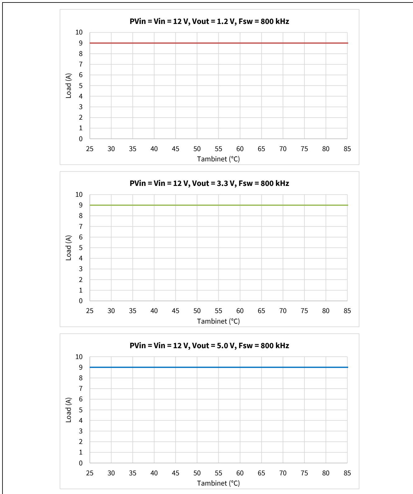
Figure 4 Thermal derating curves, P_{vin} = 12\text{ V} , V_{out} = 1.2\text{ V}/3.3\text{ V}/5\text{ V} , f_{sw} = 800\text{ kHz} , V_{CC} = \text{Internal LDO}
