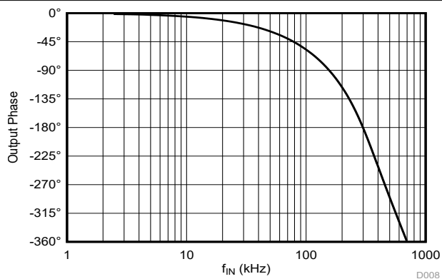
Figure 6-36. Output Phase vs Input Frequency
