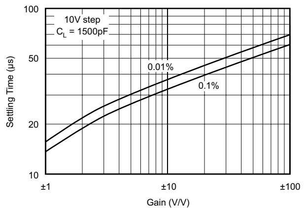
Figure 6-16. Settling Time vs Closed-Loop Gain
