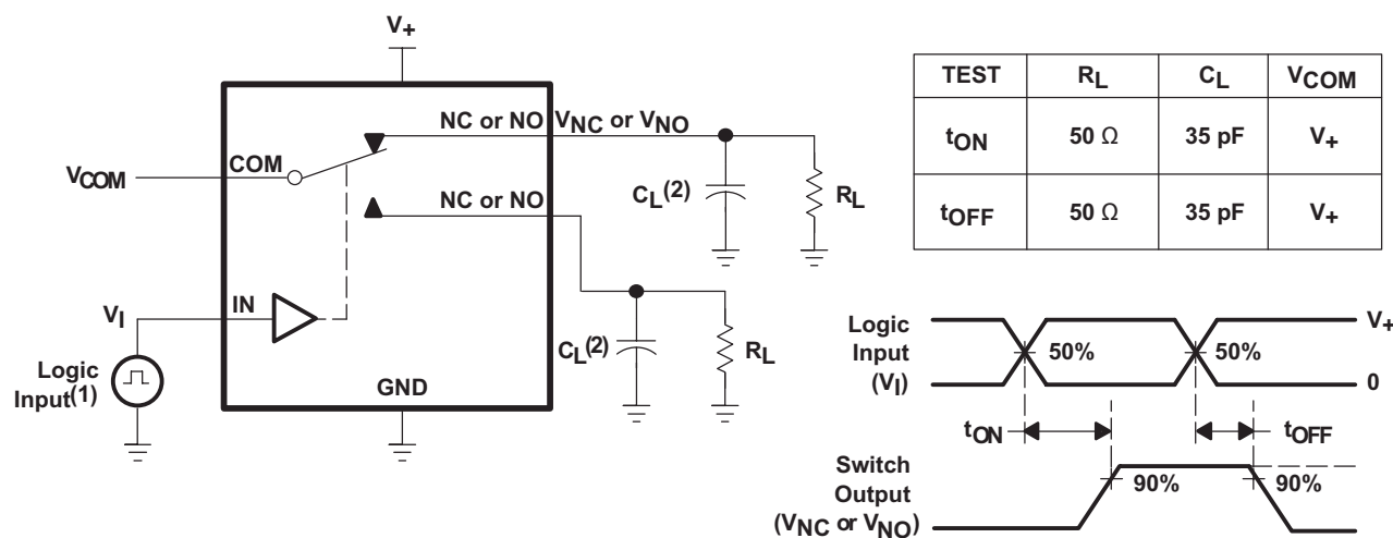
Figure 13. Capacitance (C I , C COM(ON) , C NC(OFF) , C NO(OFF) , C NC(ON) , C NO(ON) )
