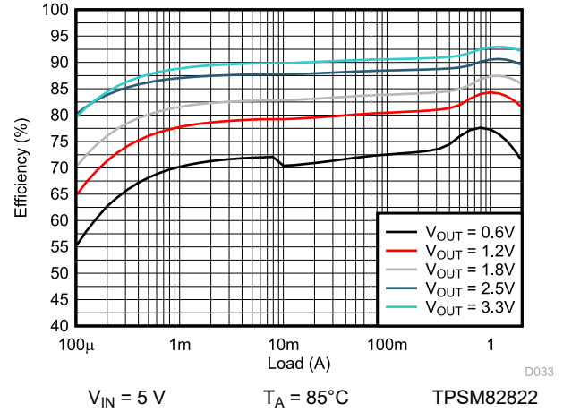
Figure 9-54. Efficiency
