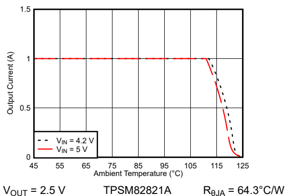
Figure 9-40. Safe Operating Area
