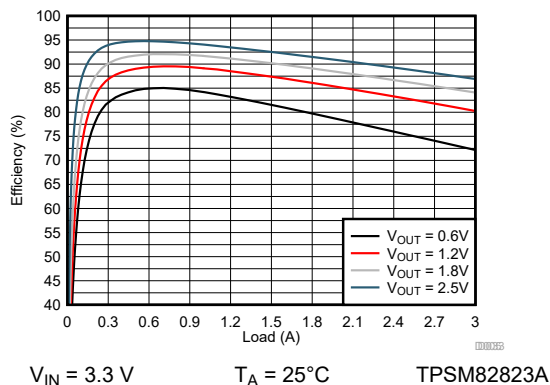
Figure 9-141. Efficiency
