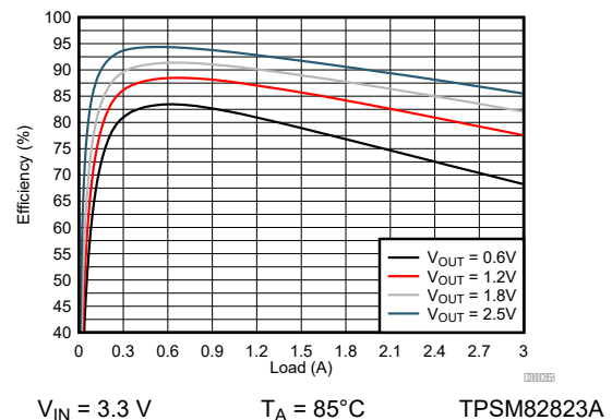
Figure 9-142. Efficiency
