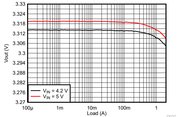
Figure 9-101. Load Regulation
