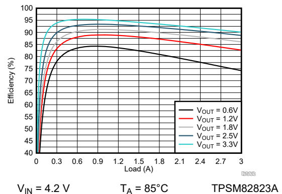
Figure 9-140. Efficiency
