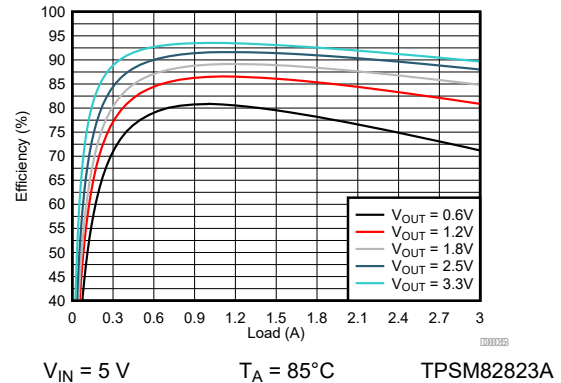
Figure 9-138. Efficiency
