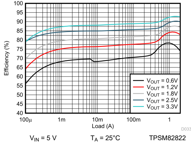
Figure 9-53. Efficiency
