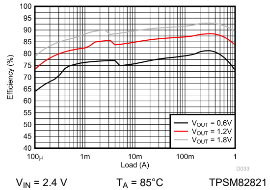
Figure 9-10. Efficiency
