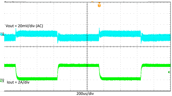
Figure 7-21. TPS563206 Load Transient With 0.3A to 2.7A
