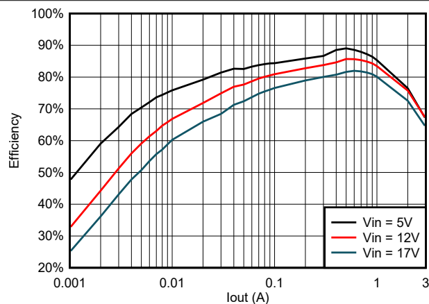
Figure 5-10. TPS563203 Efficiency at 0.6 Vout With 1.5uH Inductor
