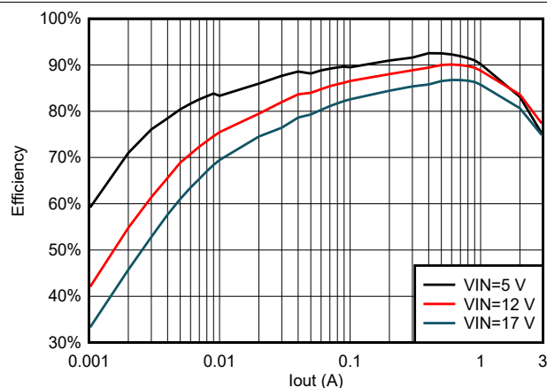
Figure 5-12. TPS563203 Efficiency at 1.05 Vout With 2.2uH Inductor
