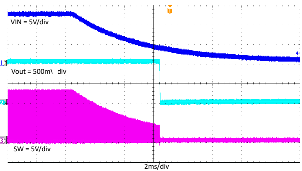
Figure 7-19. TPS563206 Power off With 3A Loading
