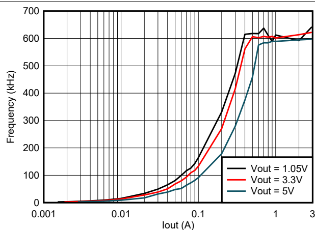
Figure 5-8. TPS563203 Frequency vs Loading
