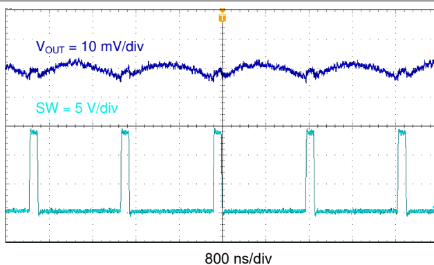
Figure 7-10. TPS563208 Output Voltage Ripple, I_{OUT} = 0 A
