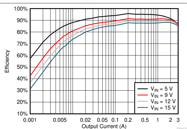
Figure 5-12. TPS563201 V_{OUT} = 3.3\text{ V} Efficiency, L = 2.2\text{ }\mu\text{H}
