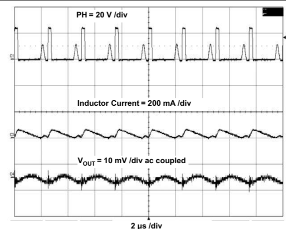
Figure 35. Output Ripple in DCM
