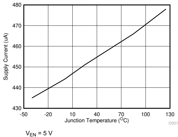
Figure 6-1. Supply Current vs Junction Temperature
