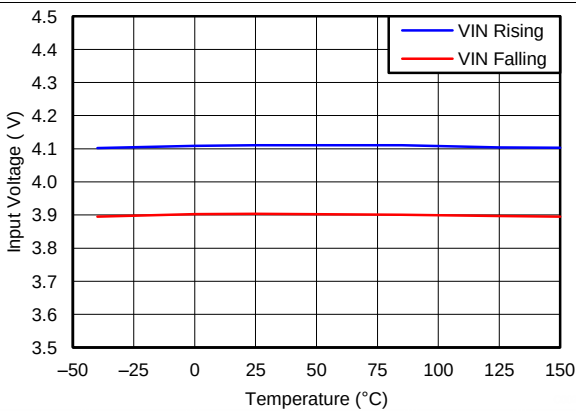
Figure 1. Input Start and Stop Voltage vs Temperature
