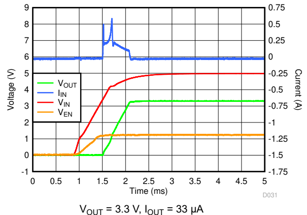
Figure 7-34. Startup Inrush Current With C_{OUT} = 47\text{ }\mu\text{F}
