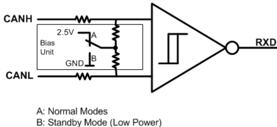
Figure 9-3. Bias Unit (Recessive Common Mode Bias) and Receiver
