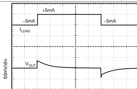
200μs/div C_L = 1\text{ }\mu\text{F} , \pm 5\text{-mA} Output Pulse
