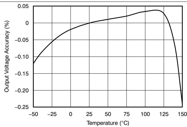
Figure 1. Temperature Drift
