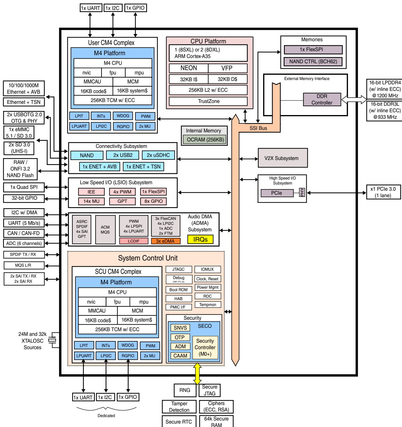
Figure 1. i.MX 8X Lite System Block Diagram
