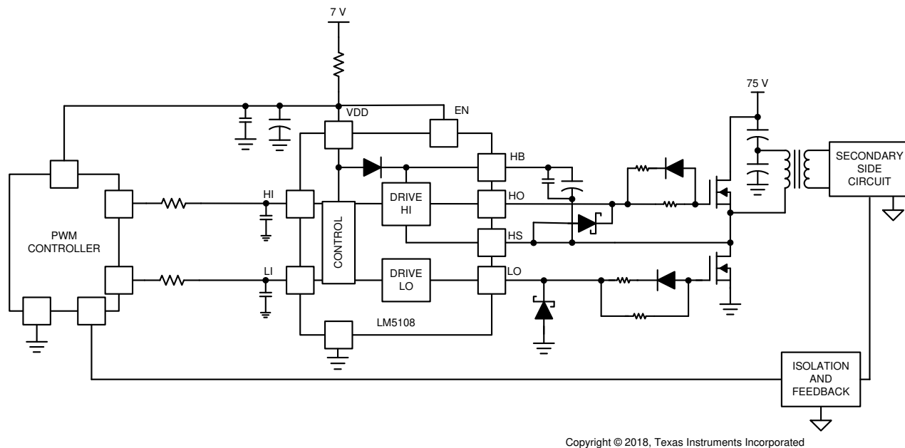
Figure 8-1. Typical Application
