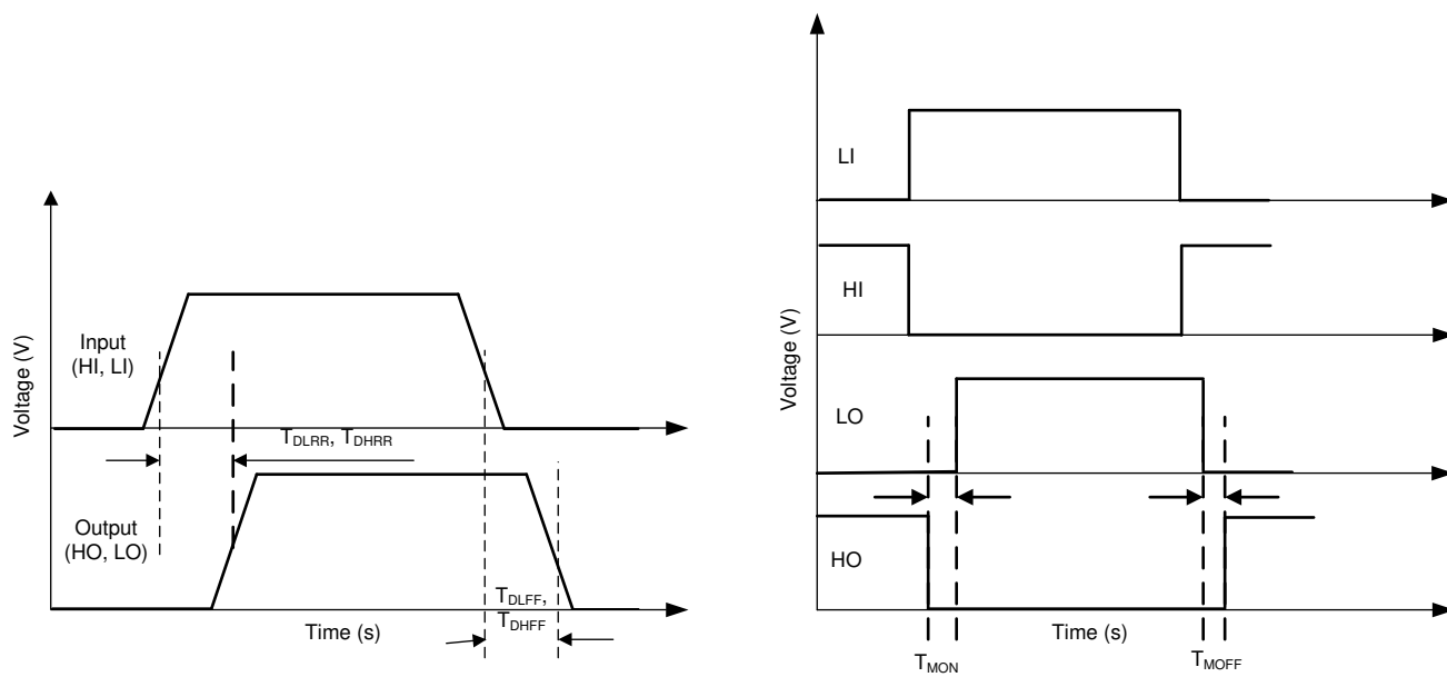
Figure 6-1. Timing Diagram
