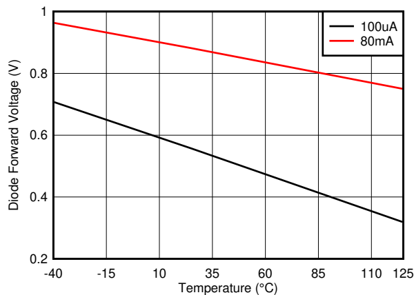
Figure 6-14. Boot Diode Forward Voltage Drop
