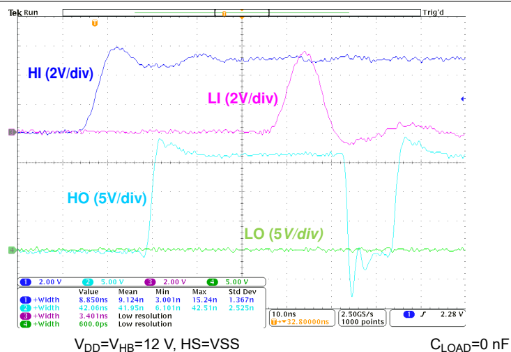
Figure 8-8. Shoot-through Protection or Interlock
