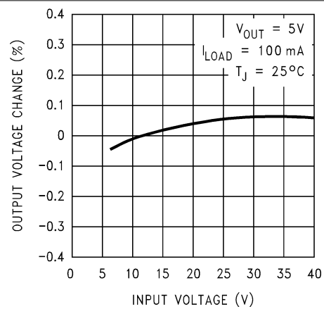
Figure 7-2. Line Regulation
