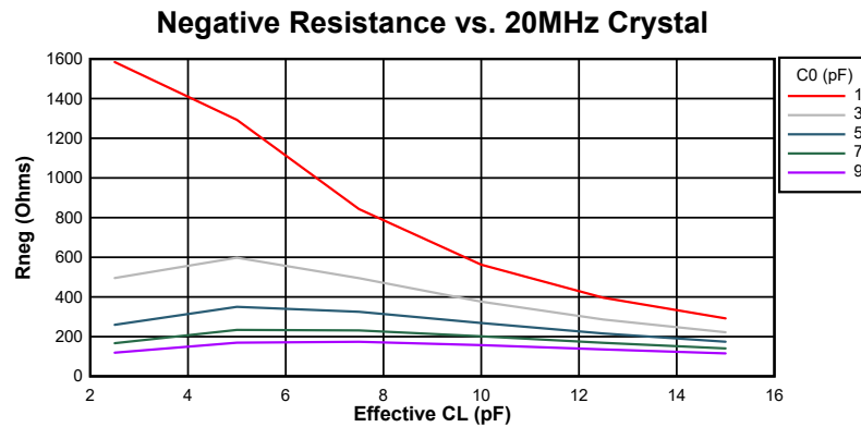
Figure 6-21. Negative Resistance Variation at 20 MHz
