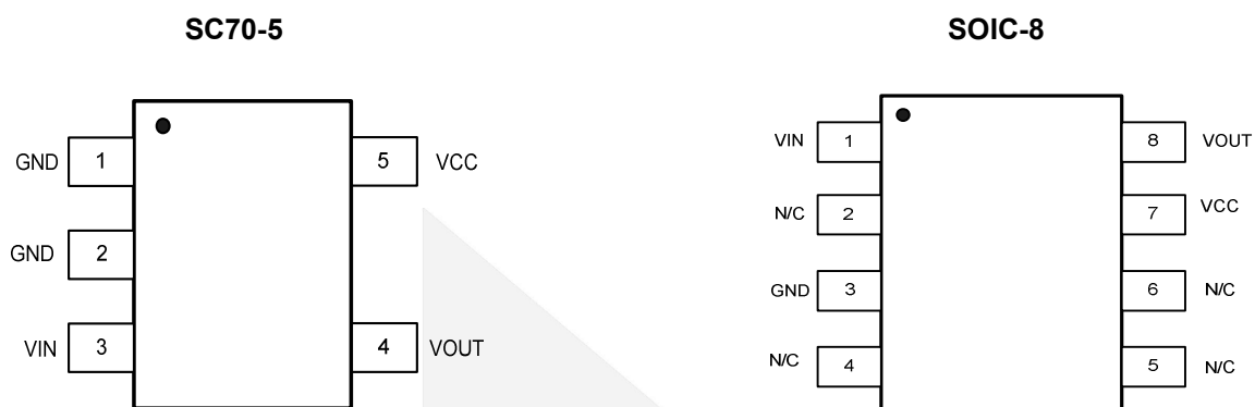
Figure 1 Pin Assignment
