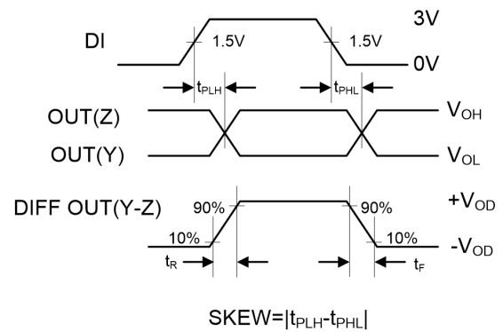
Figure 11B. Measurement Points
