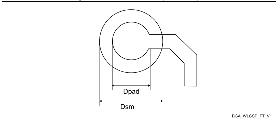
Figure 86. UFBGA169 - Footprint example
