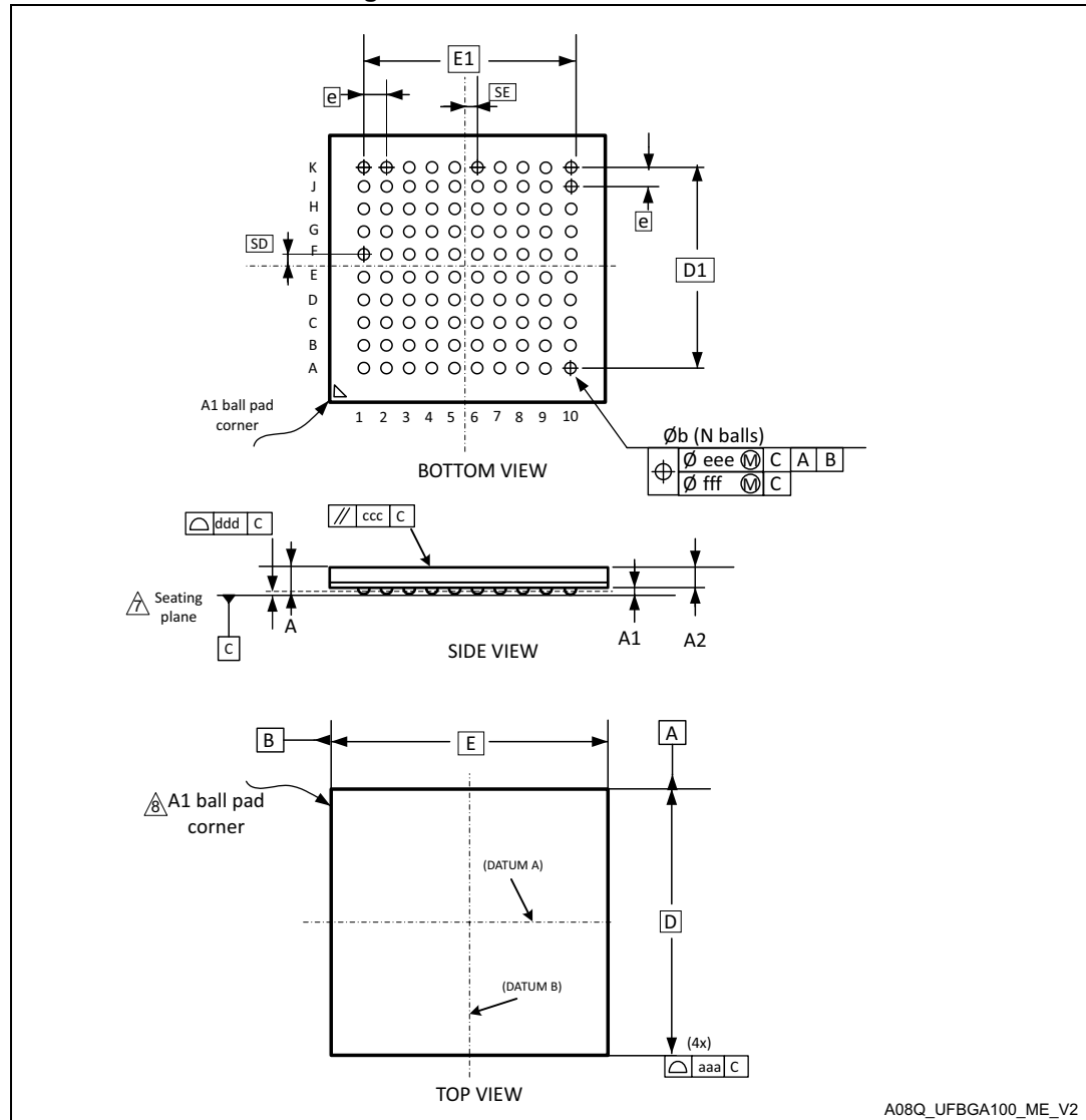
Figure 76. TFBGA100 - Outline (13)
