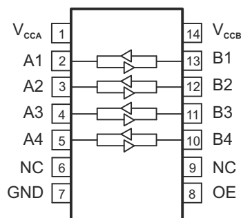
Figure 4-4. D/PW/DYY Package, 14-Pin SOIC/TSSOP/SOT (Top View)
