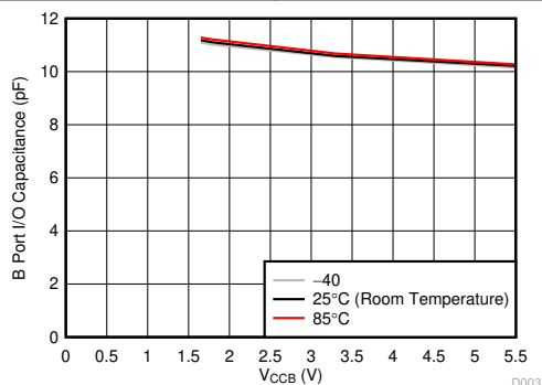
Figure 5-3. Capacitance for B Port I/O Pins ( C_{IO} ) vs Power Supply ( V_{CCB} )
