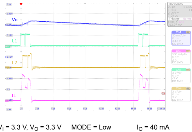
Figure 10-16. Switching Waveforms, PFM Buck-Boost Operation
