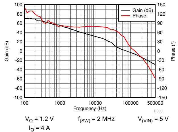
Figure 8-13. Closed-Loop Response
