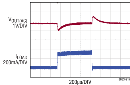
Transient Response from 18V IN to 36V OUT
