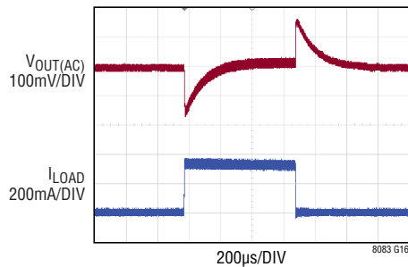
Transient Response from 36V IN to 12V OUT
