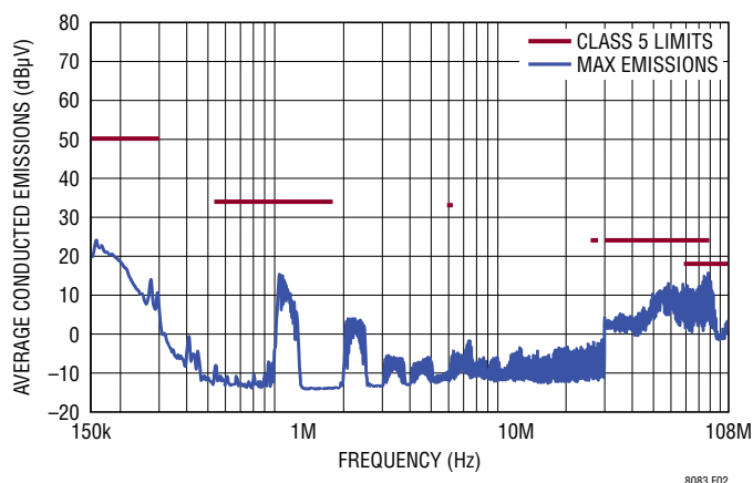
Figure 2. CISPR25 Average Conducted EMI
