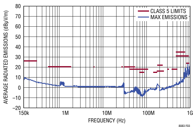
Figure 3. CISPR25 Average Radiated EMI
