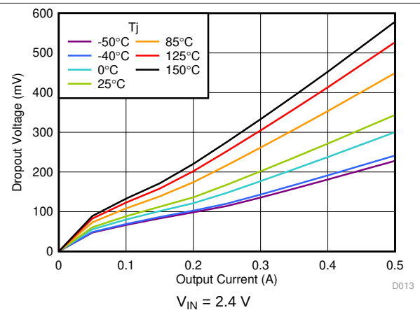
Figure 6. Dropout Voltage vs I_{OUT}
