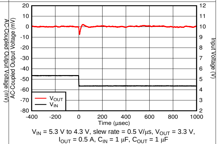
Figure 30. Line Transient
