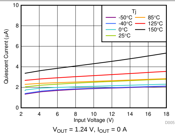
Figure 10. I_Q vs V_{IN}
