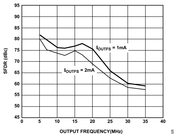
Figure 31. SFDR vs. f_{OUT} and I_{OUTFS} at 80 MSPS
