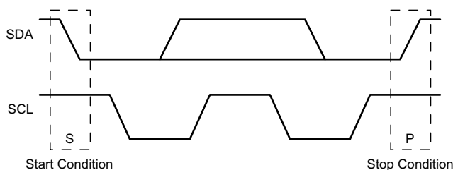
Figure 8-22. I²C Definition of Start and Stop Conditions
