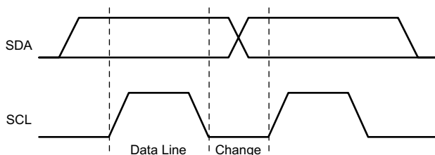
Figure 8-23. I²C Bit Transfer
