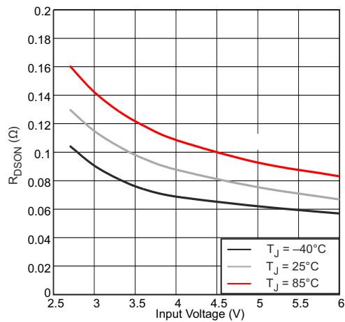
Figure 7-5. Static Drain-Source On-State Resistance vs Input Voltage
