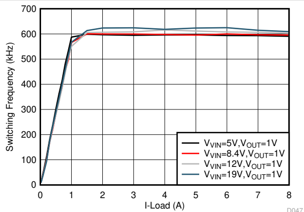
Figure 8-3. Load Regulation, F_{sw} = 600\text{ kHz}
