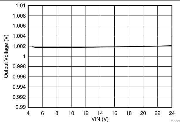
Figure 8-6. Line Regulation, I_{OUT} = 0.01\text{ A}
