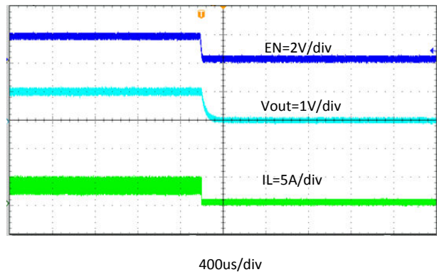
Figure 8-11. Shut-down Through EN, I_{OUT} = 4 A
