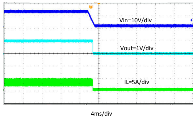
Figure 8-13. Start Up Relative to V_{IN} Falling, I_{OUT} = 4 A
