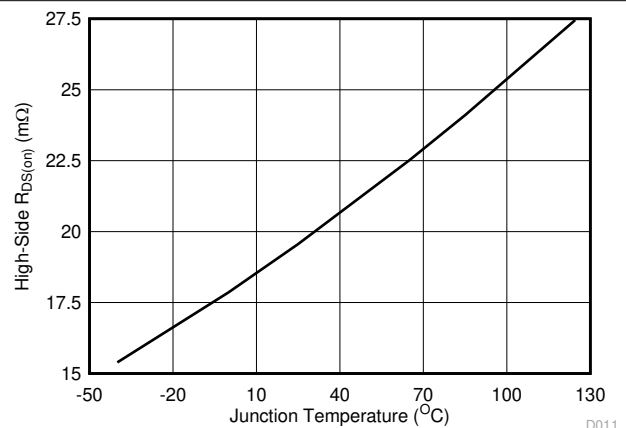
Figure 6-6. High-Side R_{DS(on)} vs Junction Temperature
