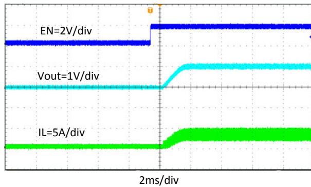
Figure 8-10. Start-Up Through EN, I_{OUT} = 4 A
