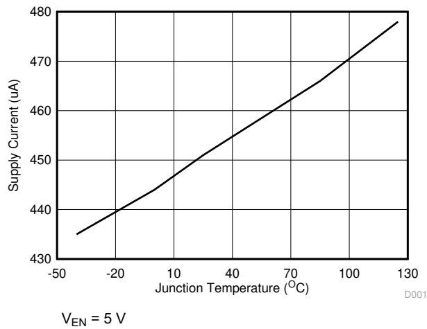
Figure 6-1. Supply Current vs Junction Temperature
