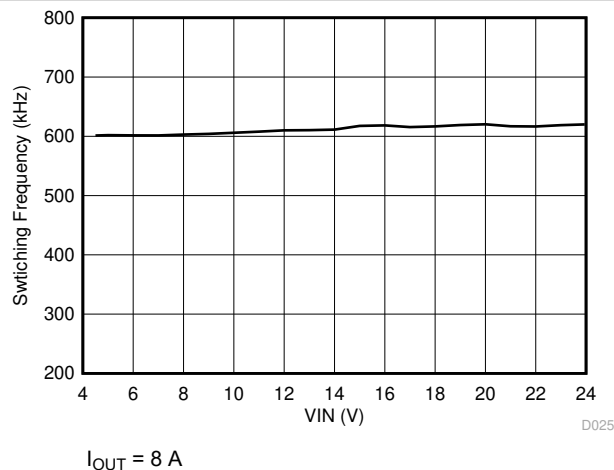
Figure 8-4. Switching Frequency vs Input Voltage
