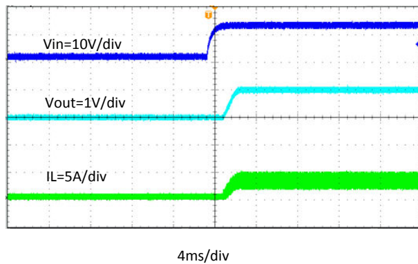
Figure 8-12. Start Up Relative to V_{IN} Rising, I_{OUT} = 4 A
