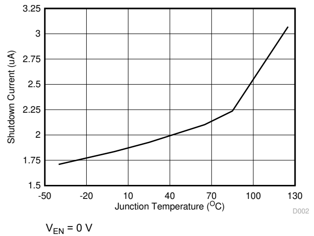
Figure 6-2. Shutdown Current vs Temperature
