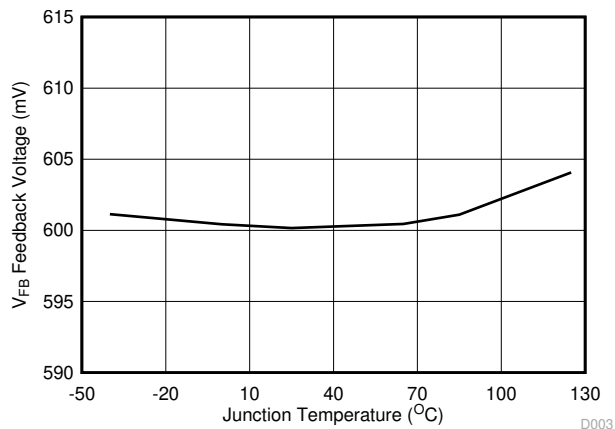
Figure 6-3. Feedback Voltage vs Junction Temperature
