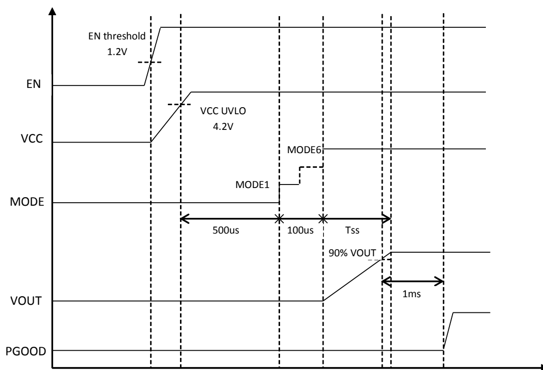
Figure 7-1. Power-Up Sequence
