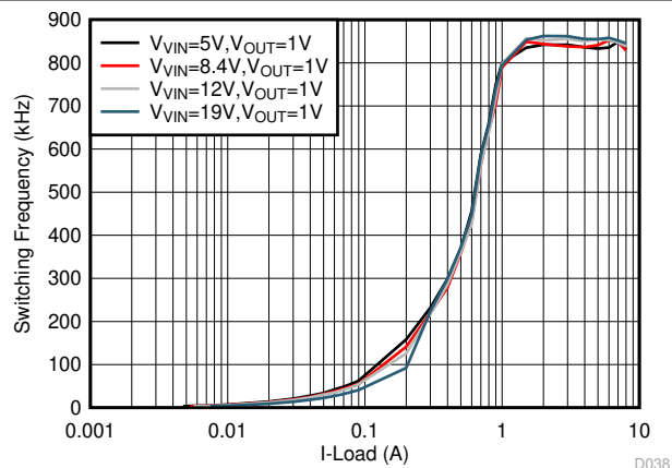
Figure 6-19. F_{SW} Load Regulation, Eco-mode, F_{SW} = 800 kHz
