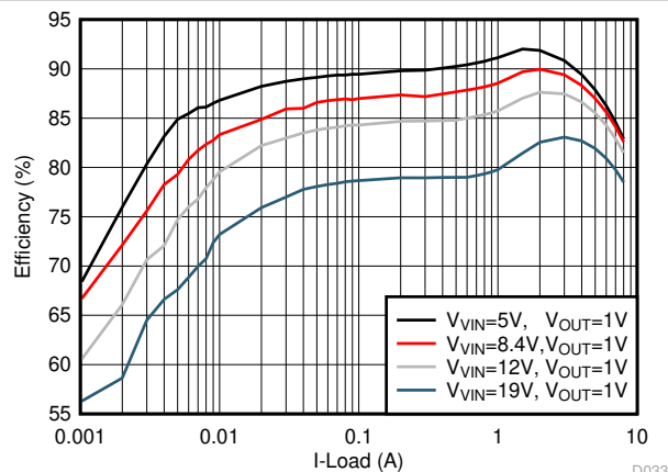
Figure 8-2. Efficiency Curve, F_{sw} = 600\text{ kHz}
