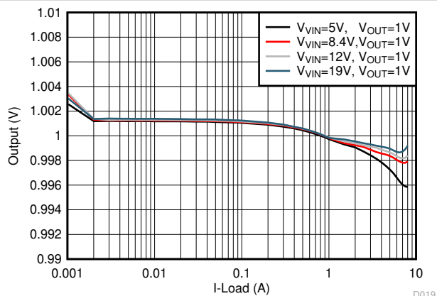
Figure 8-3. Load Regulation, F_{sw} = 600\text{ kHz}
