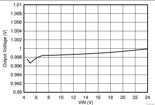
Figure 8-7. Line Regulation, I_{OUT} = 8\text{ A}
