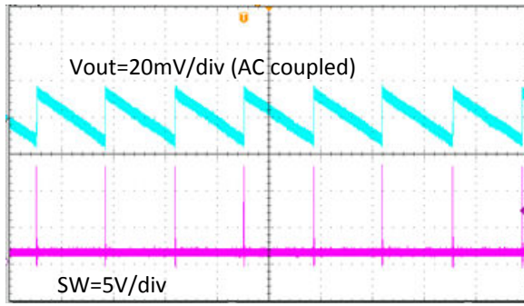
Figure 8-8. Output Voltage Ripple, I_{OUT} = 0.01 A
