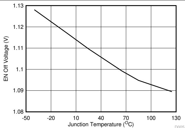
Figure 6-5. Enable Off Voltage vs Junction Temperature
