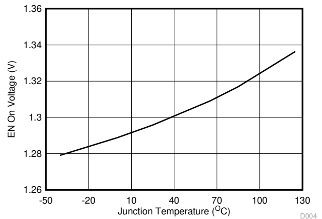
Figure 6-4. Enable On Voltage vs Junction Temperature
