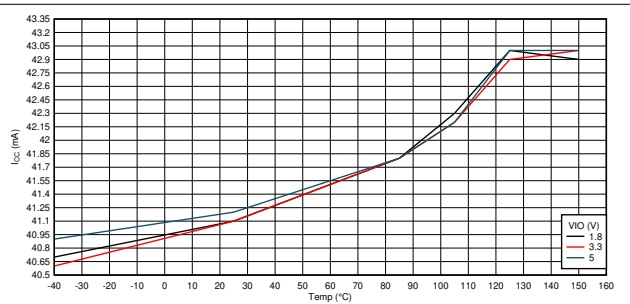
Figure 11-9. Normal Mode: I_{CC} vs Temperature Dominant
