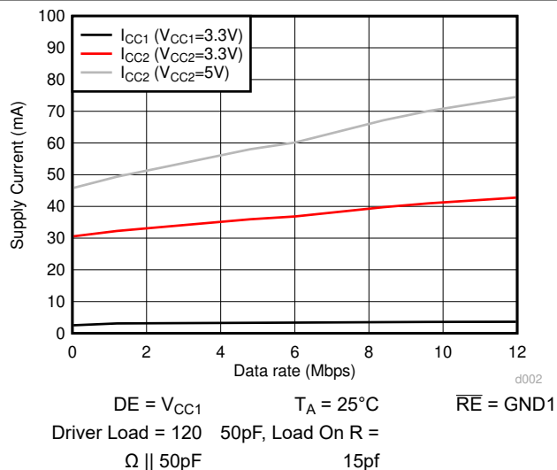
Figure 7-7. ISO143x Supply Current Vs. Data Rate - 120\Omega||50\text{pF} Load
