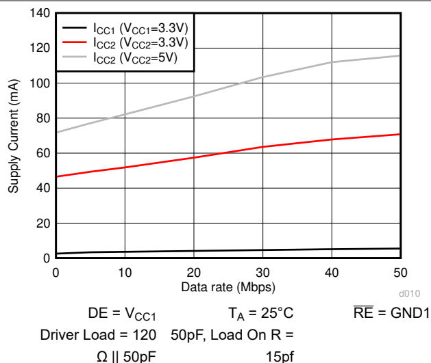
Figure 7-10. ISO145x Supply Current Vs Data Rate- 120\Omega||50\text{pF} Load
