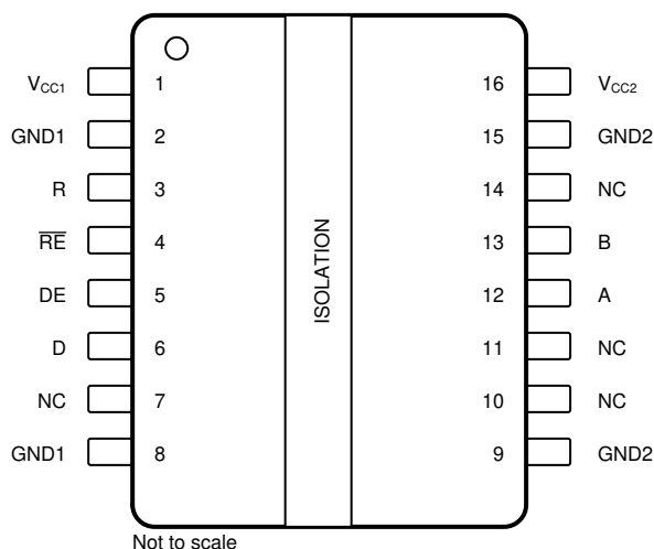
Figure 6-2. DW Package 16-Pin SOIC Half-Duplex Device Top View
