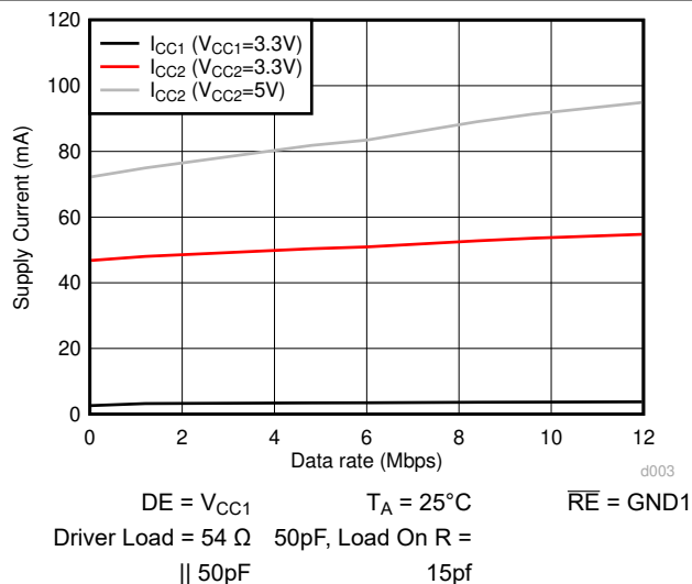
Figure 7-8. ISO143x Supply Current Vs Data Rate- 54\Omega||50\text{pF} Load
