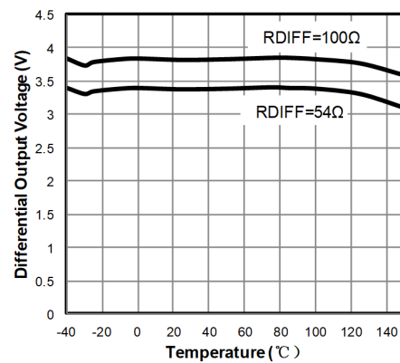
Figure 2. Driver Differential Output Voltage vs. Temperature
