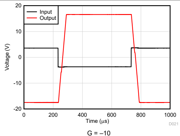
Figure 5-28. Overload Recovery
