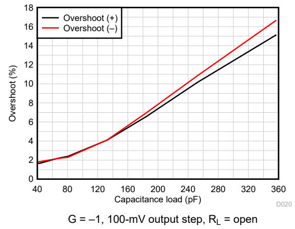
Figure 5-26. Small-Signal Overshoot vs Capacitive Load
