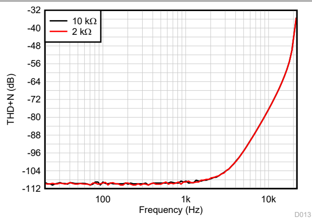
Figure 5-18. THD+N Ratio vs Frequency, G = 1 G = 1 , f = 1\text{ kHz} , BW = 80\text{ kHz} , V_{OUT} = 10\text{ V}_{PP} , R_L connected to V_-
