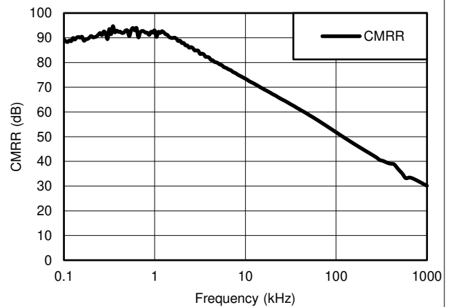
Figure 5-42. Common-Mode Rejection Ratio vs Frequency
