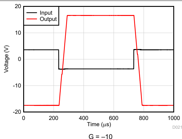
Figure 5-28. Overload Recovery
