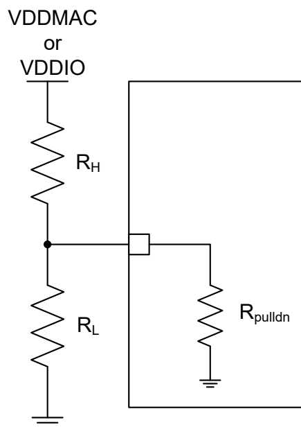
Figure 8-18. Strap Circuit
