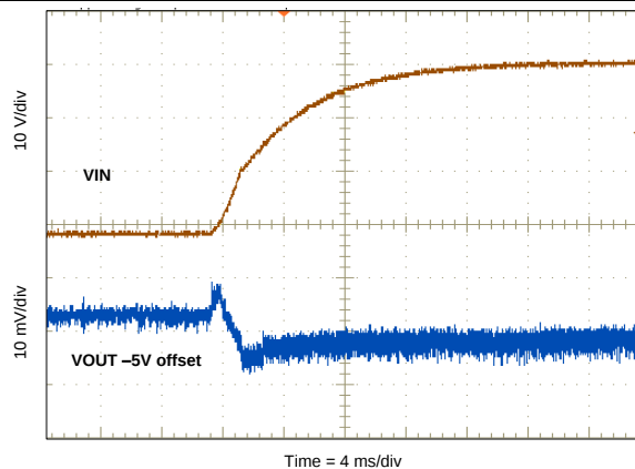
Figure 35. Line Transient (8 V to 40 V)
