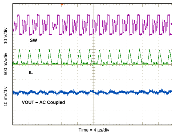
Figure 39. Output Ripple DCM
