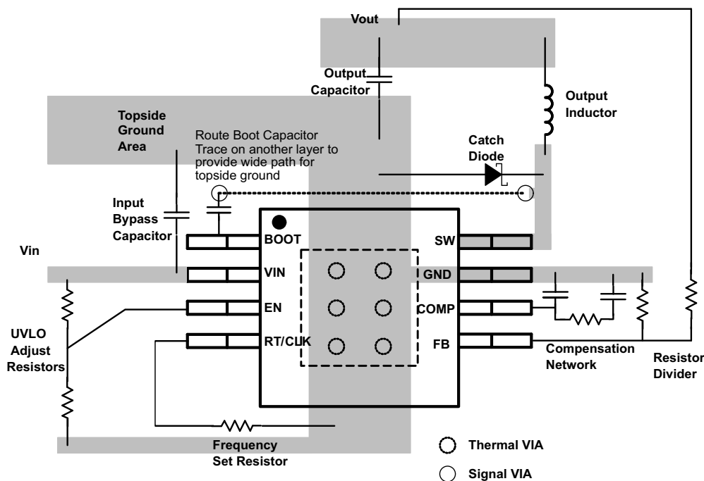
Figure 58. PCB Layout Example
