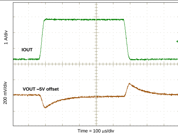
Figure 34. Load Transient
