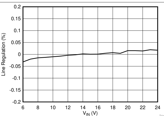
Figure 8-6. Line Regulation, I_{OUT} = 0.1\text{ A}
