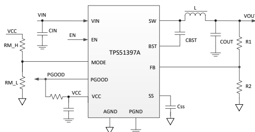
Simplified Schematic
