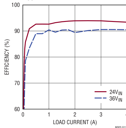
Efficiency vs Load Current, V_{OUT} = -8\text{V} , BIAS Tied to LTM8003 GND
