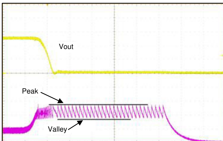
Figure 7-1. Current Limit Operation During Output Short Circuit
