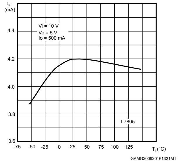
Figure 33. Quiescent current vs junction temp.
