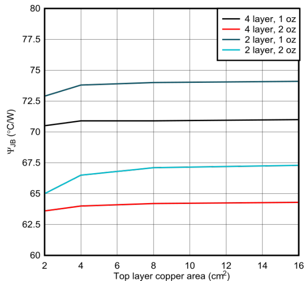
Figure 9-34. SOT, junction-to-board characterization parameter vs copper area
