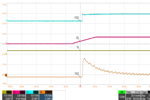
A. Channel 1 = IN1, IN2 (paralleled) Channel 2 = V_{CC} Channel 3 = V_{OUT} (OUT1/2 paralleled) Channel 8 = Motor Current
