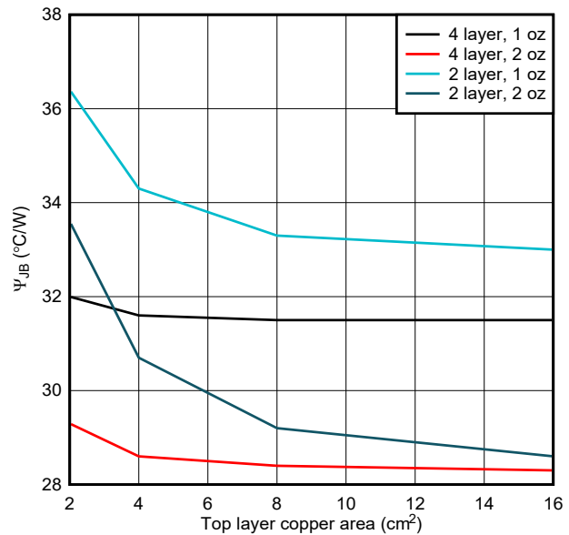
Figure 9-32. WSON, junction-to-board characterization parameter vs copper area
