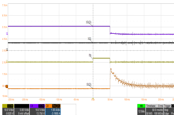
A. Channel 1 = IN1, IN2 (paralleled) Channel 5 = V_{CC} Channel 6 = V_{OUT} (OUT1/2 paralleled) Channel 8 = Motor Current
