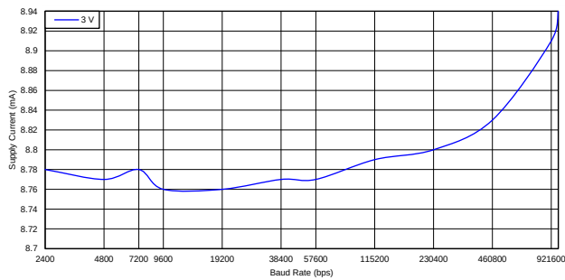
Figure 4-2. Supply Current at 3 V
