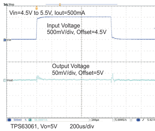
Figure 9-17. Line Transient Response
