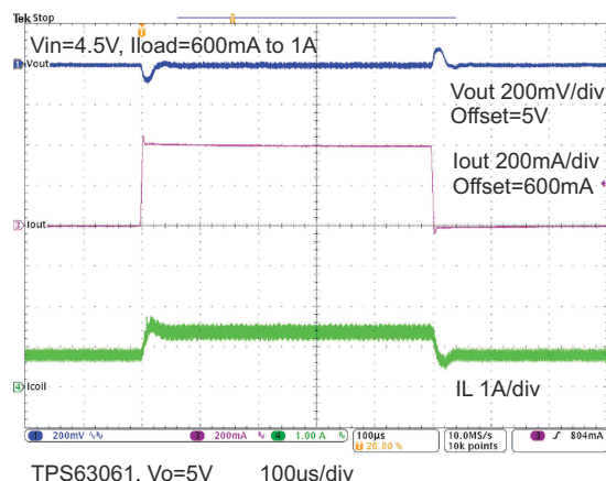
Figure 9-15. Load Transient Response
