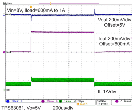
Figure 9-16. Load Transient Response
